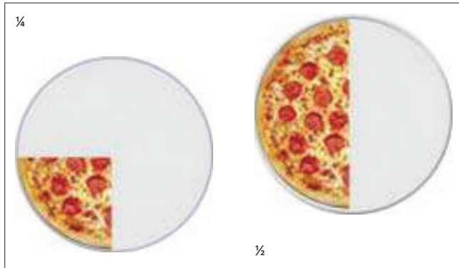
FIGURE 1: Fraction scheme.
