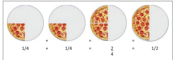
FIGURE 2: Addition and subtraction of fractions.
